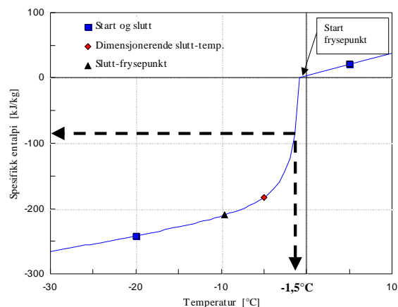
Figur 3. Entalpikurve for laks
