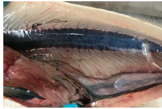
(b) Score 2.
