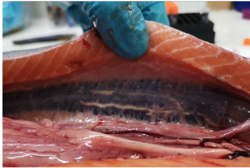
(c) Score 3.
